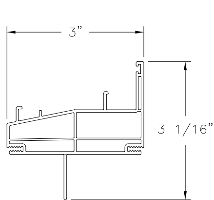
SILL FIN INSTALLATION (CH9202) EXTRUDED RIGID PVC
