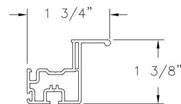
LIFT RAIL (CH9005) EXTRUDED RIGID PVC
