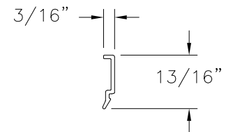
GLAZING BEAD (DT1770-R) EXTRUDED RIGID PVC
