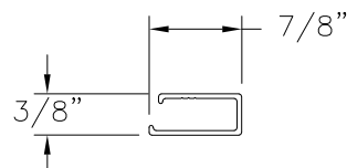
LOCK RAIL/STILE REINFORCEMENT (731-A) ALUMINUM 6063-T5
