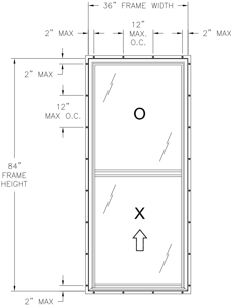
200/275 VINYL SINGLE HUNG WINDOW EXTERIOR VIEW FIN INSTALLATION
