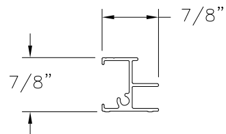
MEETING RAIL REINFORCEMENT (200A) ALUMINUM 6063-T5
