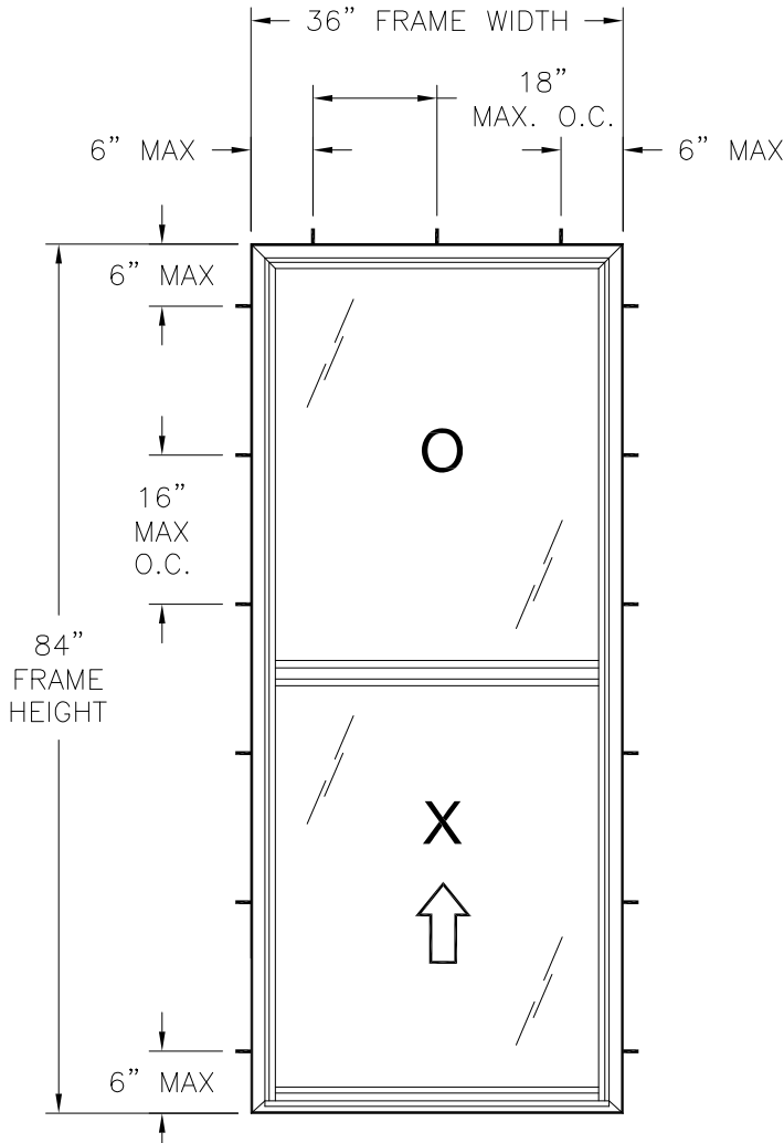
200/275 VINYL SINGLE HUNG WINDOW EXTERIOR VIEW FRAME INSTALLATION
